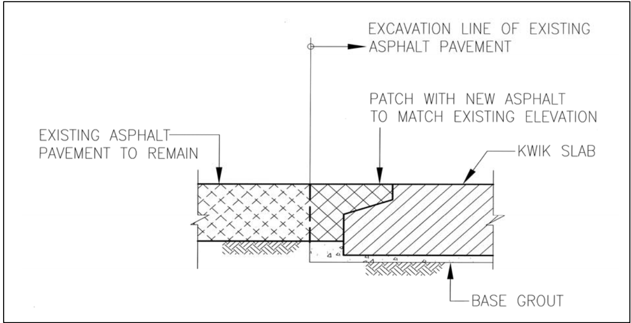
EXISTING ASPHALT PATCH WITH NEW ASPHALT KWIK SLAB
